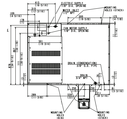
REMOTE AIR-COOLED
