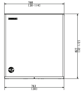
REMOTE AIR-COOLED
